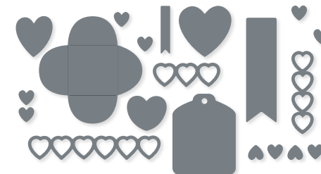
SWEET HEARTS DIES 157623 | $50.00 AUD | $61.00 NZD 16 dies. Largest die: 3-1/4" x 5/8" (8.3 x 1.6 cm).
